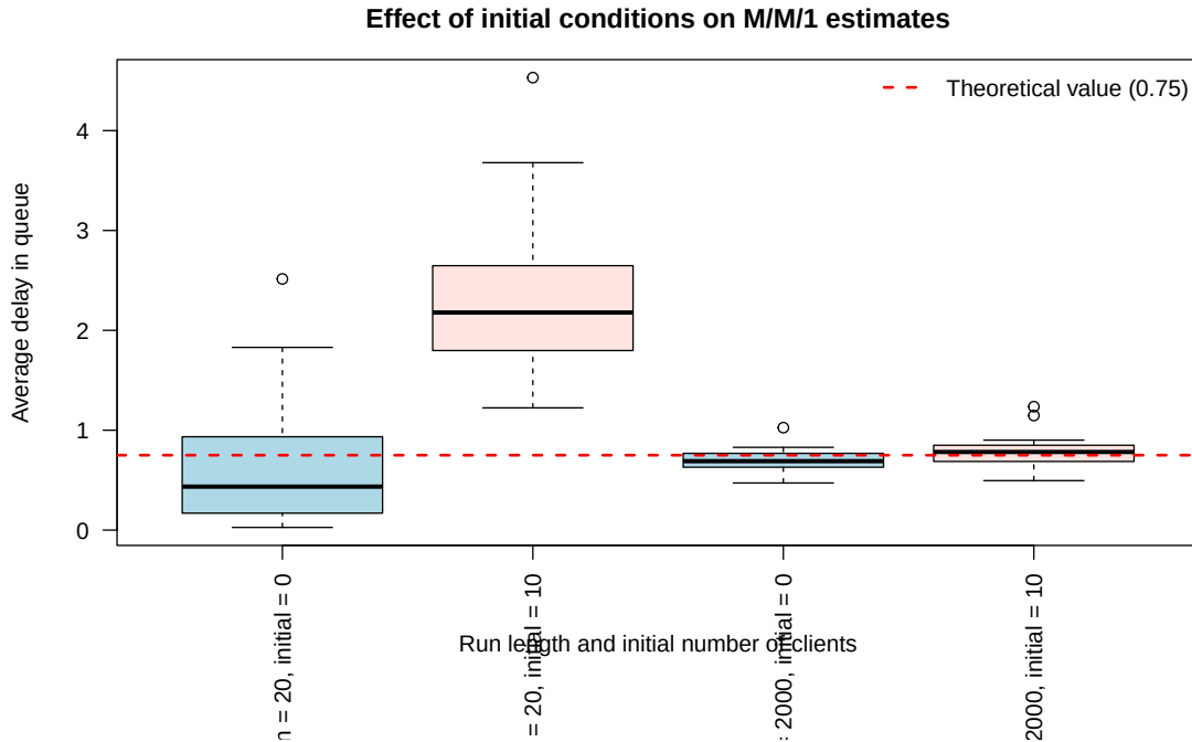
Figure 9: Distribution of the 25 average queue-delay estimates for each run length and initial condition. The dashed line marks the theoretical value W_Q = 0.75 .
