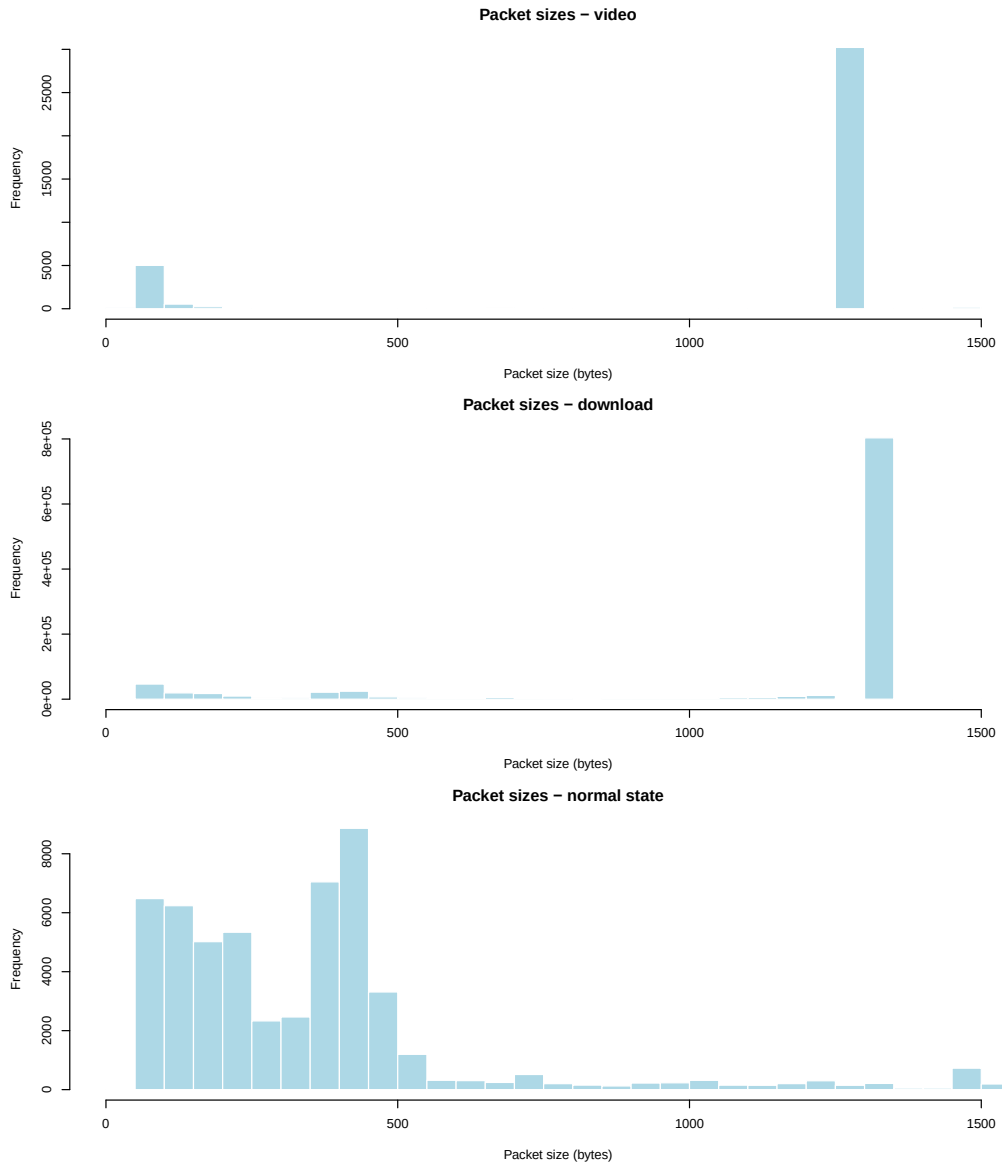
Figure 4: Packet-size histograms for the video, download, and normal-state captures, using common 50-byte bins.
