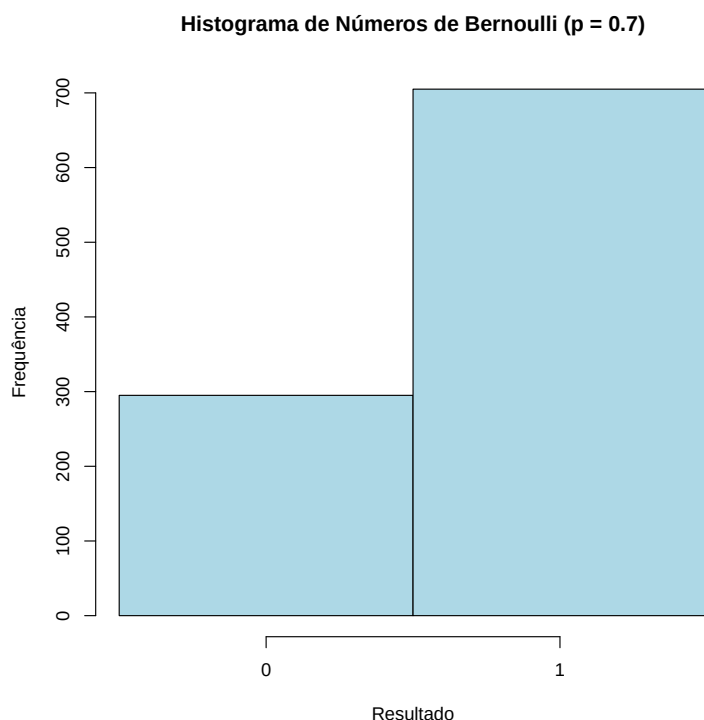
Figure 2: Histogram of 1000 Bernoulli samples with p = 0.7 .
