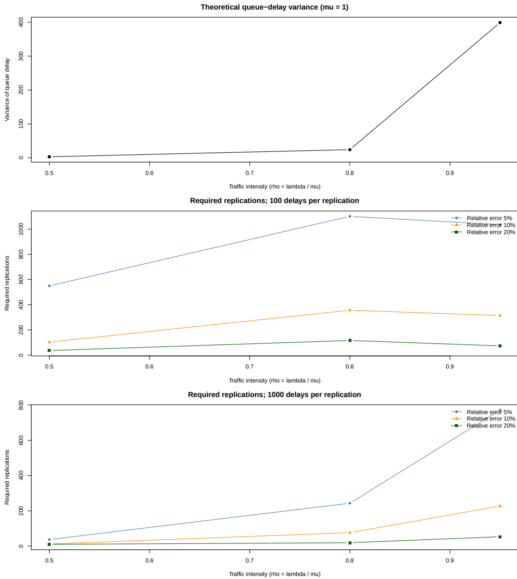
Figure 10: Theoretical queue-delay variance and observed replication requirements as functions of \rho , for two measured sample sizes.
