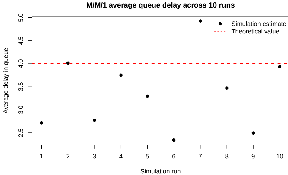
Figure 8: Average queue-delay estimate in each of the ten M/M/1 runs. The dashed line marks the theoretical value W_Q = 4 .
