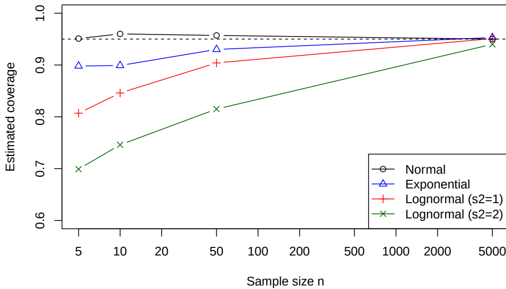
Figure 7: Estimated coverage vs. sample size n (log scale), for the four distributions. Dashed line: nominal 95% level.
