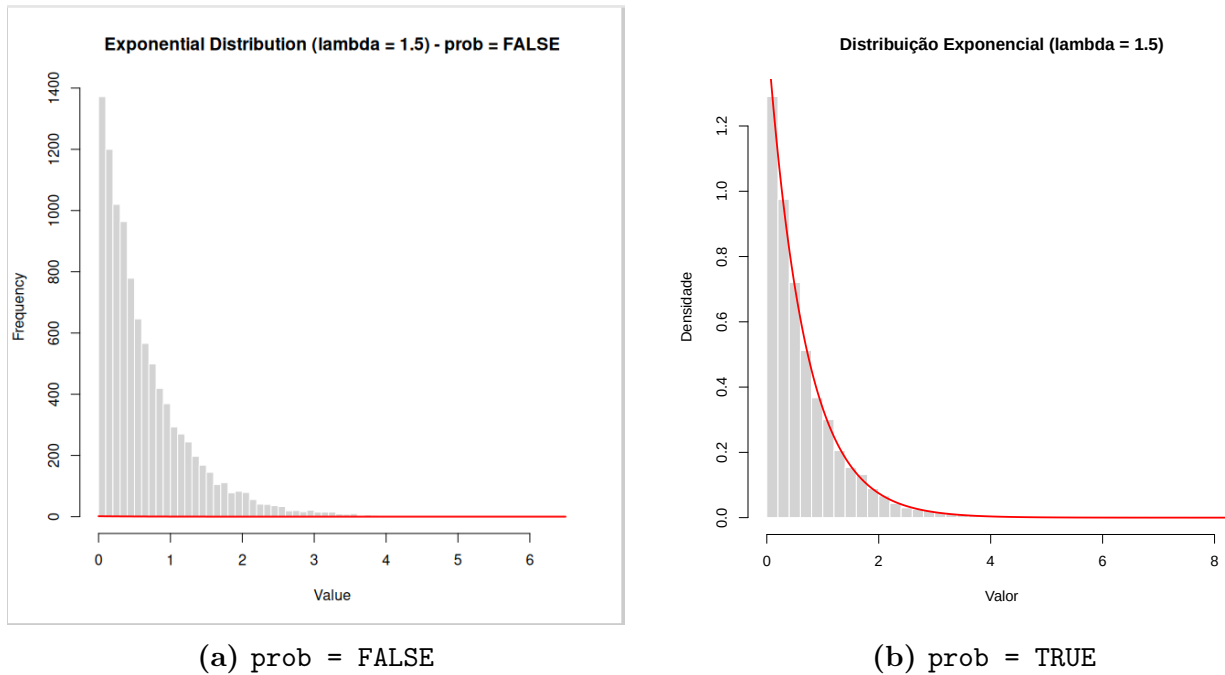
Figure 3: Histogram of 10000 exponentially distributed samples ( \lambda = 1.5 ) with the theoretical pdf (red line) superposed, with and without density normalization.
