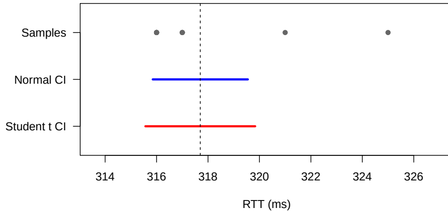
Figure 6: RTT samples and the two 95% confidence intervals (dashed line: sample mean).
